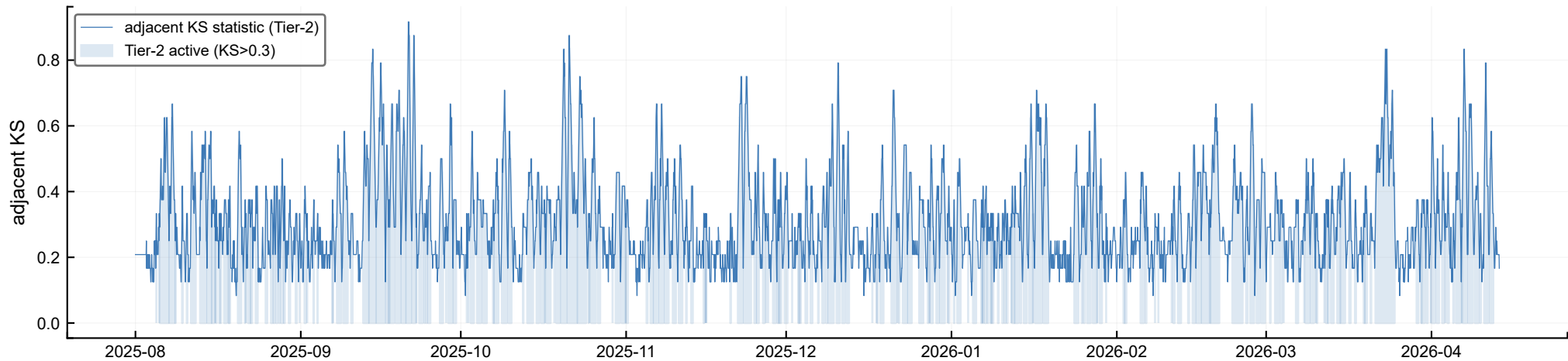
(b) Tier-2 adjacent KS — DO_2_3
